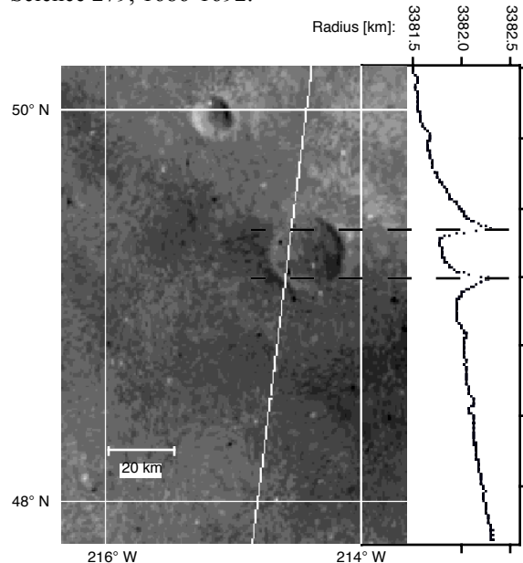
Figure Caption: Prototype map for a small area on the northern hemisphere of Mars (left) computed on the basis of the updated "Viking control point network". A laser altimeter profile across a crater obtained by MOLA (Mars Orbiter Laser Altimeter) from board the Mars Global Surveyor is used to verify the geometric accuracy of this map. The topographic data acquired by MOLA are shown on the right, while the corresponding laser surface reflection points, as given in MOLA experiment ancillary data sets, are plotted on the map. The precise match between instrument and map data, as the MOLA surface track intersects a crater, indicate that the Mars-fixed coordinate system and the map are correctly tied to within the spatial resolution of the map of 1 km.
